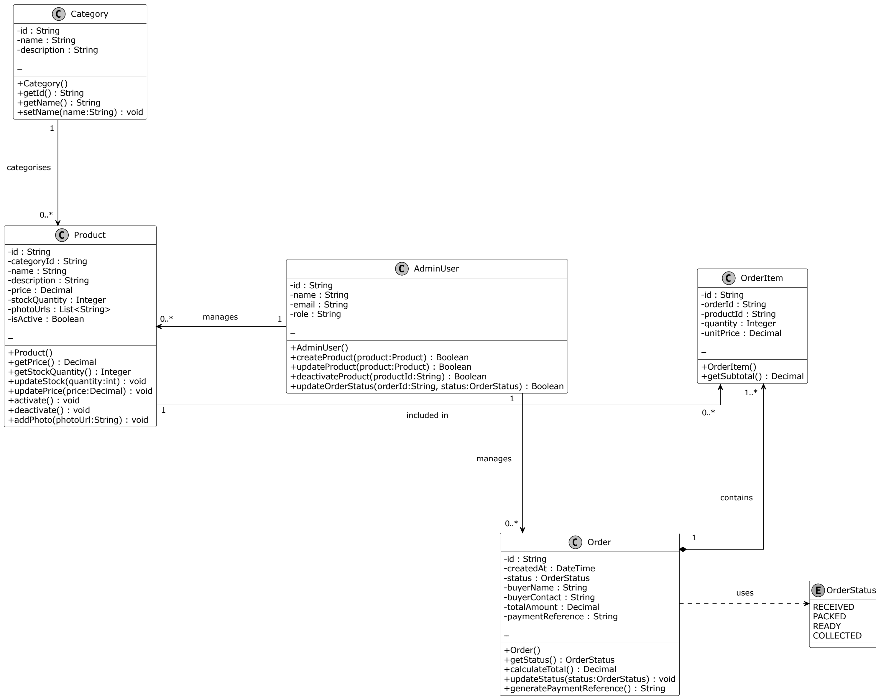
Design Class Diagram (Implementation Level)
